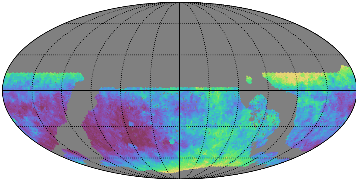
ddf_loaded_half_fl4_v3.4_10yrs WFD z band: Median seeingEff
