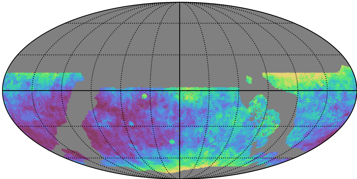
ddf_loaded_half_fl4_v3.4_10yrs WFD y band: Median seeingEff
