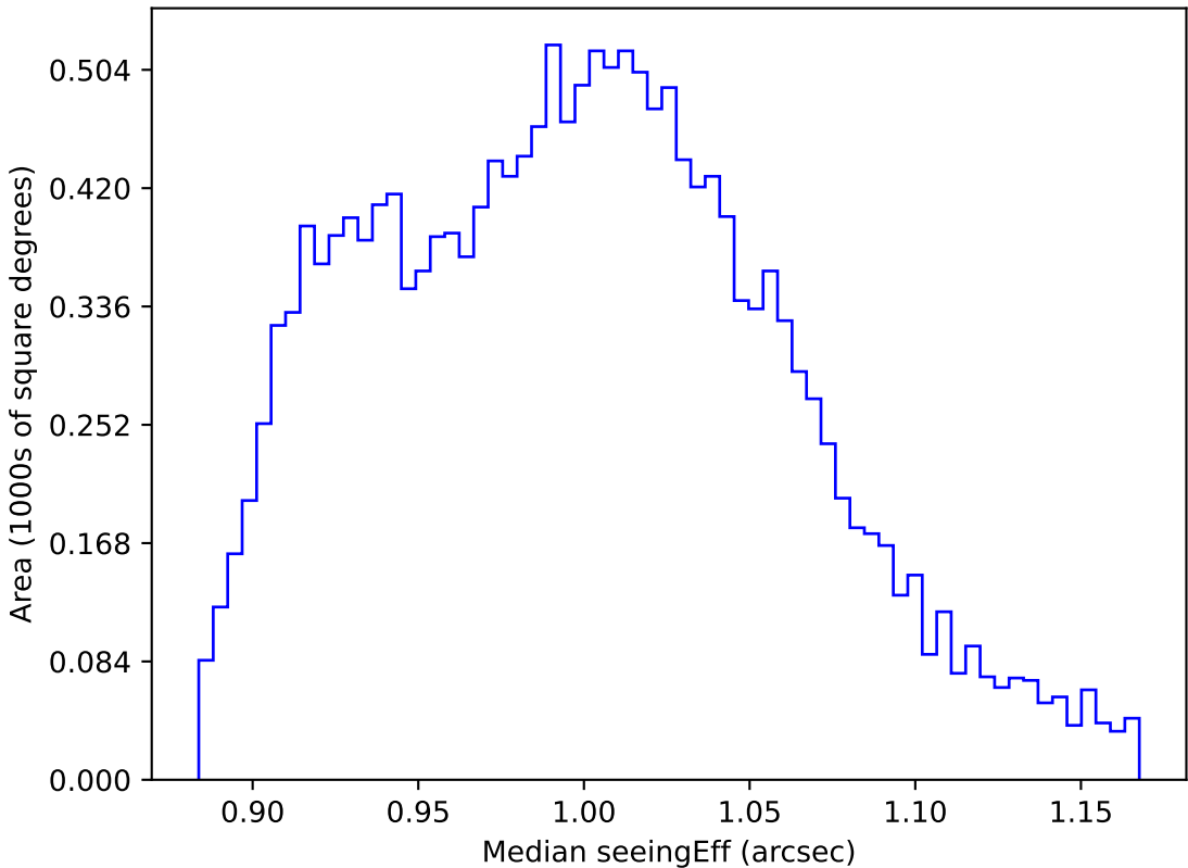
ddf_loaded_half_fl4_v3.4_10yrs WFD y band: Median seeingEff
