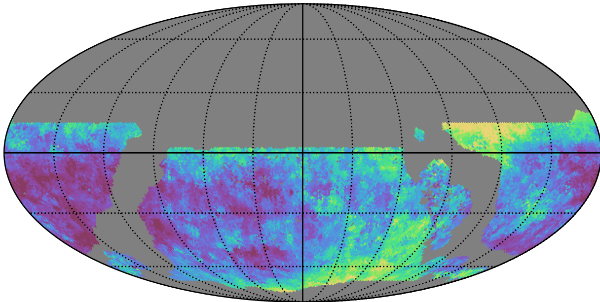
ddf_loaded_half_fl4_v3.4_10yrs WFD u band: Median seeingEff
