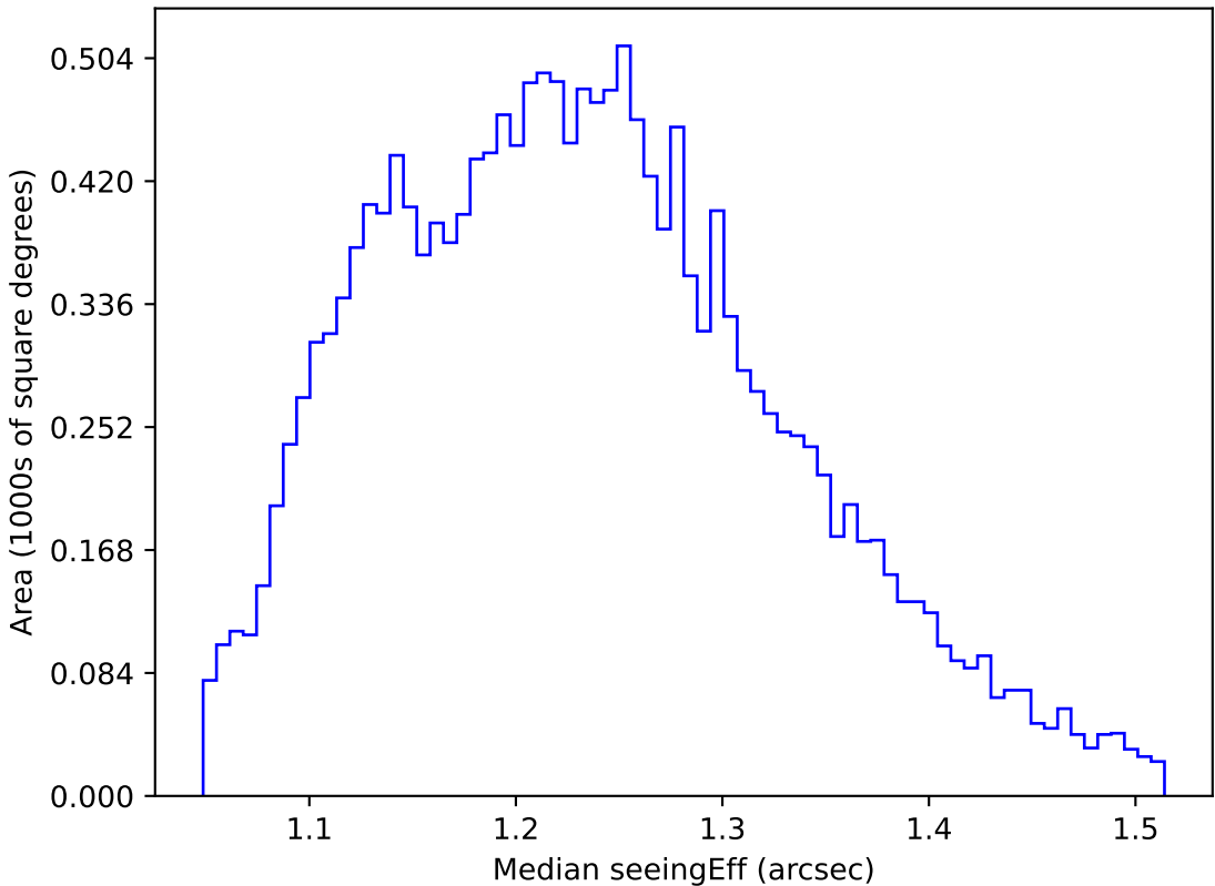
ddf_loaded_half_fl4_v3.4_10yrs WFD u band: Median seeingEff
