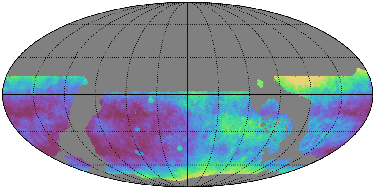
ddf_loaded_half_fl4_v3.4_10yrs WFD r band: Median seeingEff
