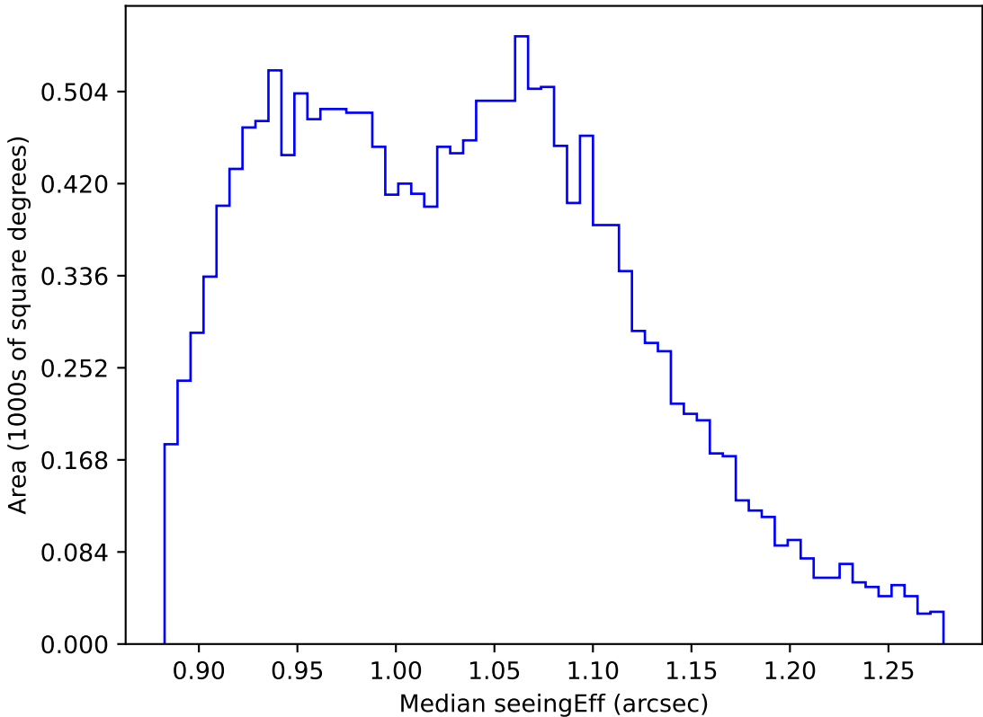
ddf_loaded_half_fl4_v3.4_10yrs WFD r band: Median seeingEff
