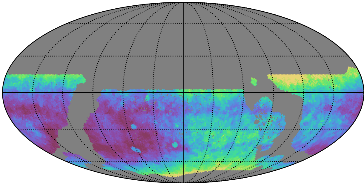
ddf_loaded_half_fl4_v3.4_10yrs WFD i band: Median seeingEff
