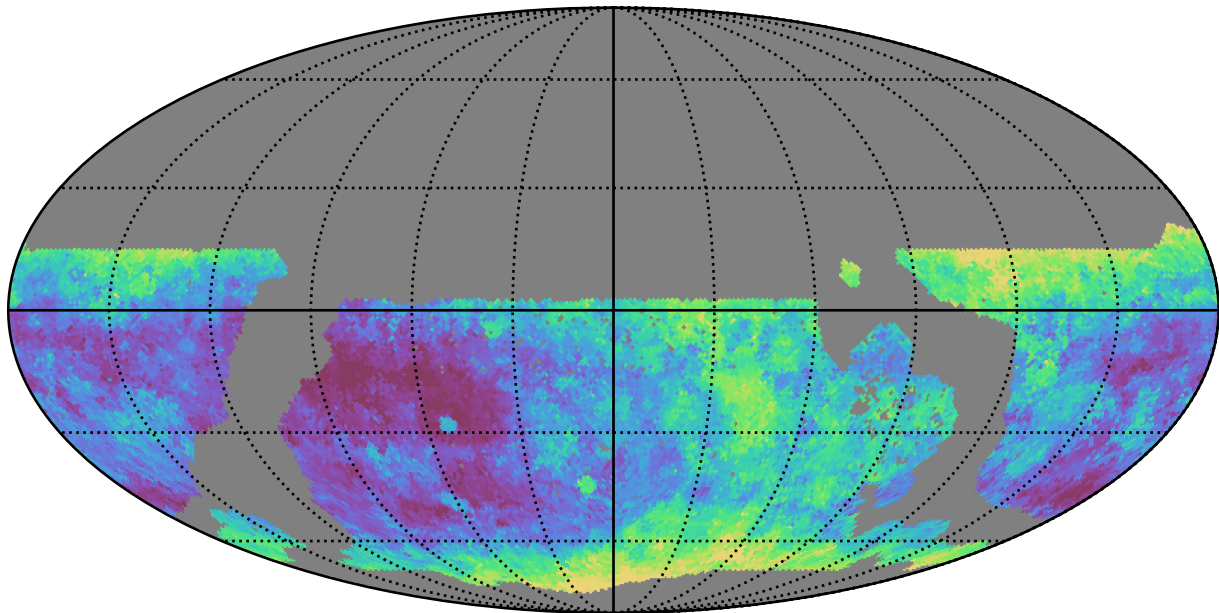
ddf_loaded_half_fl4_v3.4_10yrs WFD g band: Median seeingEff
