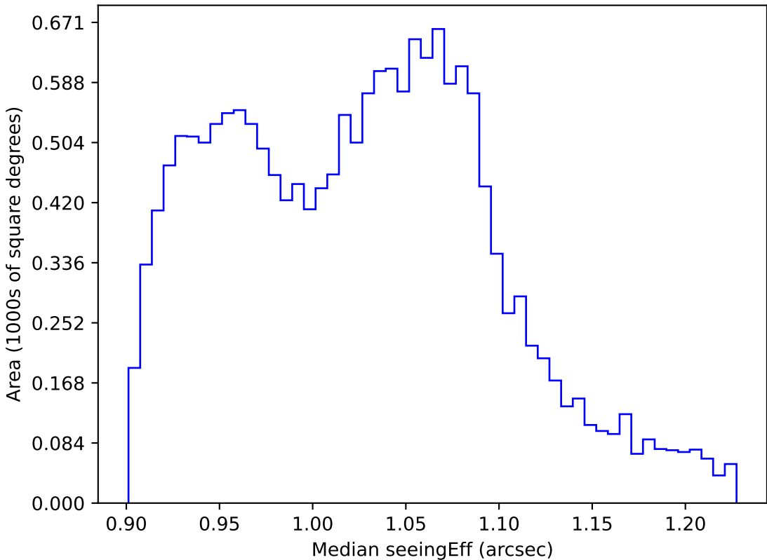
ddf_loaded_half_f14_v3.4_10yrs WFD all bands: Median seeingEff
