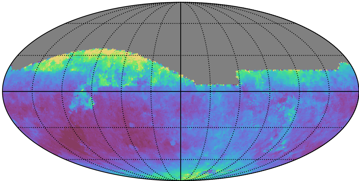
ddf_loaded_half_fl4_v3.4_10yrs All sky z band: Median seeingEff
