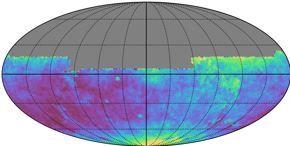
ddf_loaded_half_fl4_v3.4_10yrs All sky y band: Median seeingEff
