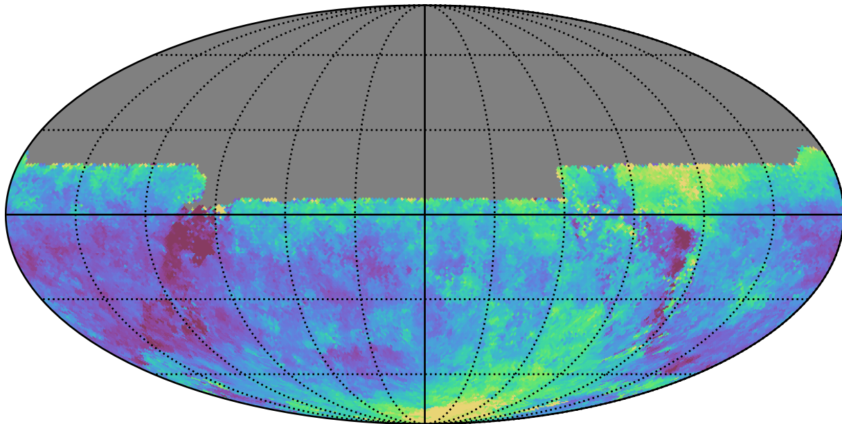
ddf_loaded_half_fl4_v3.4_10yrs All sky u band: Median seeingEff
