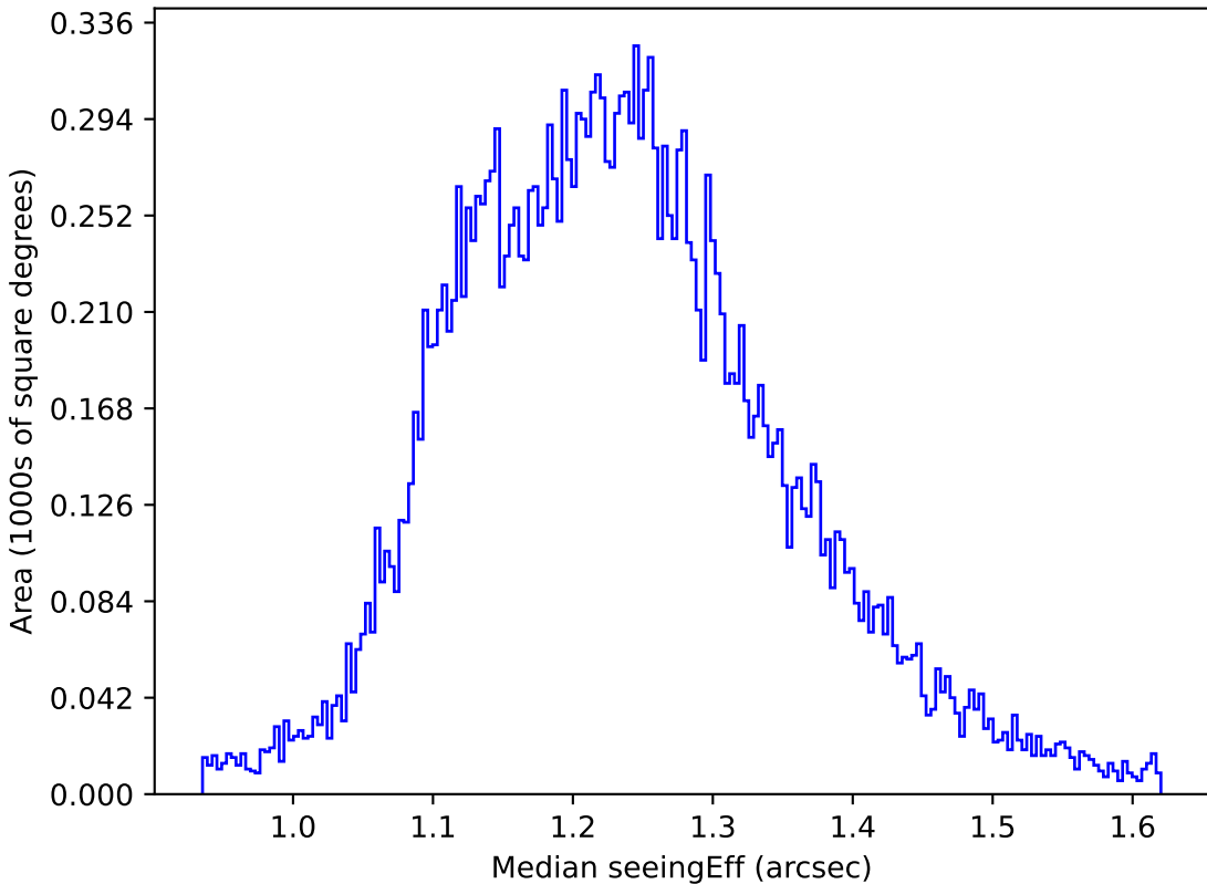
ddf_loaded_half_fl4_v3.4_10yrs All sky u band: Median seeingEff
