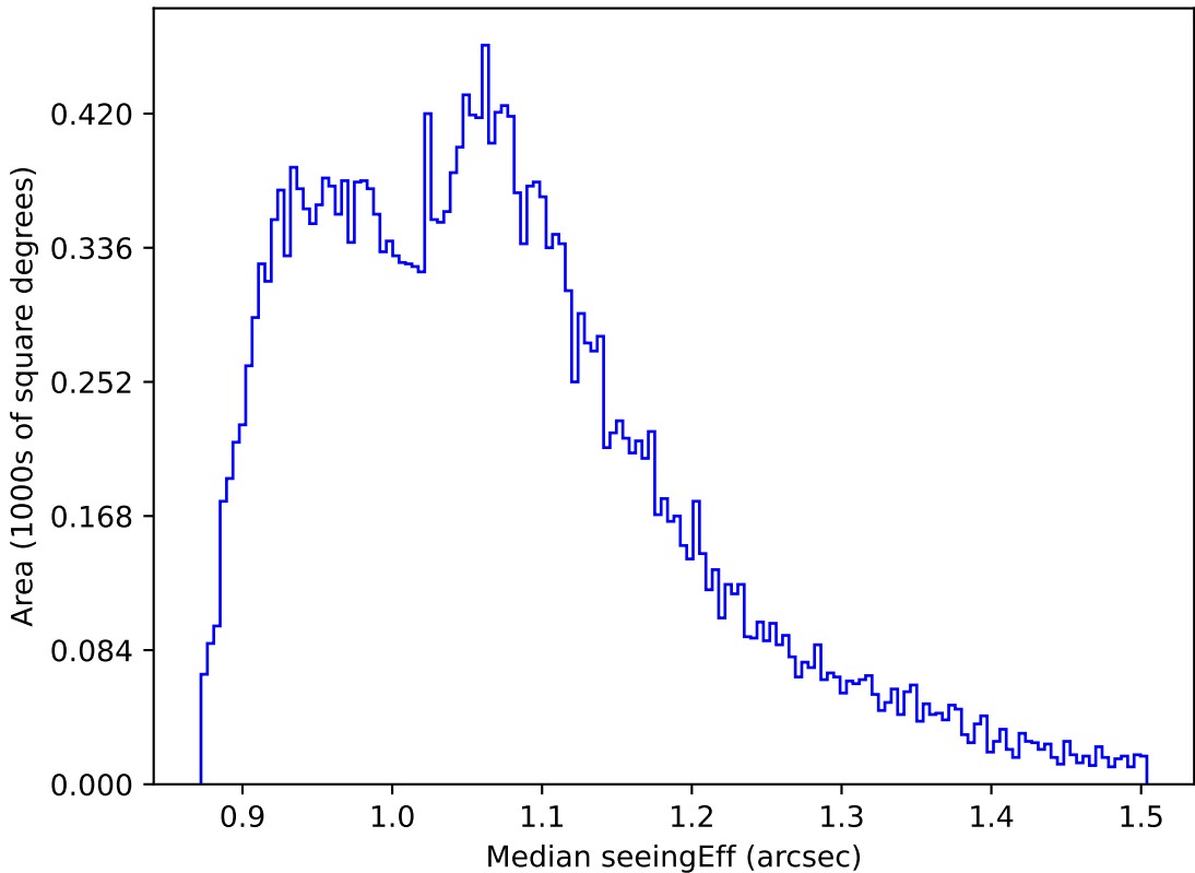
ddf_loaded_half_fl4_v3.4_10yrs All sky r band: Median seeingEff
