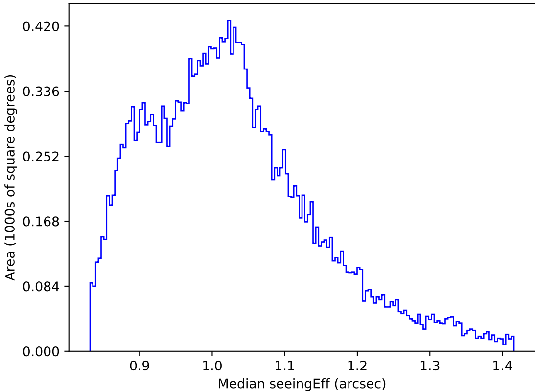
ddf_loaded_half_fl4_v3.4_10yrs All sky i band: Median seeingEff
