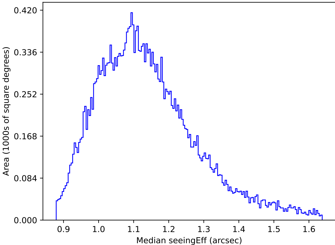
ddf_loaded_half_fl4_v3.4_10yrs All sky g band: Median seeingEff
