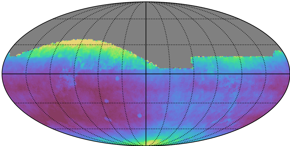
ddf_loaded_half_fl4_v3.4_10yrs All sky all bands: Median seeingEff
