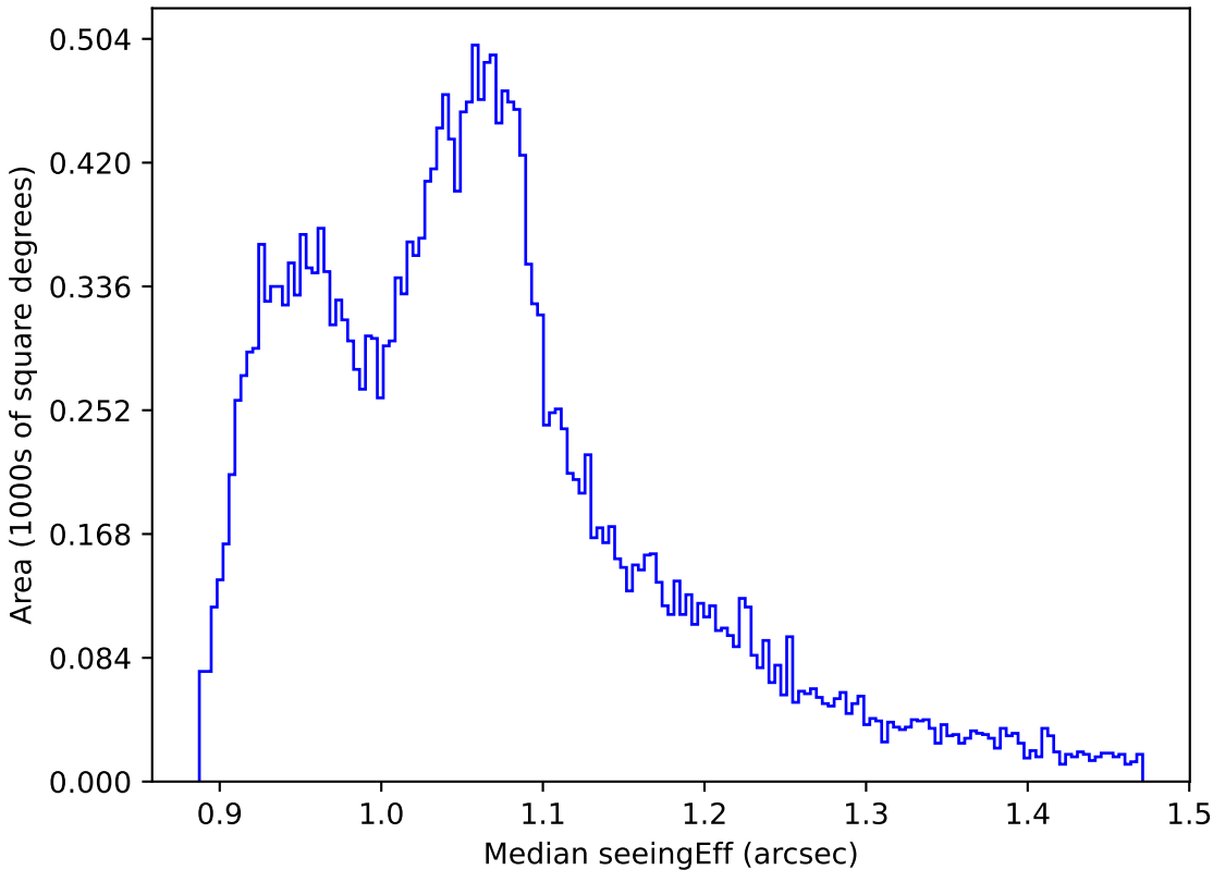
ddf_loaded_half_fl4_v3.4_10yrs All sky all bands: Median seeingEff
