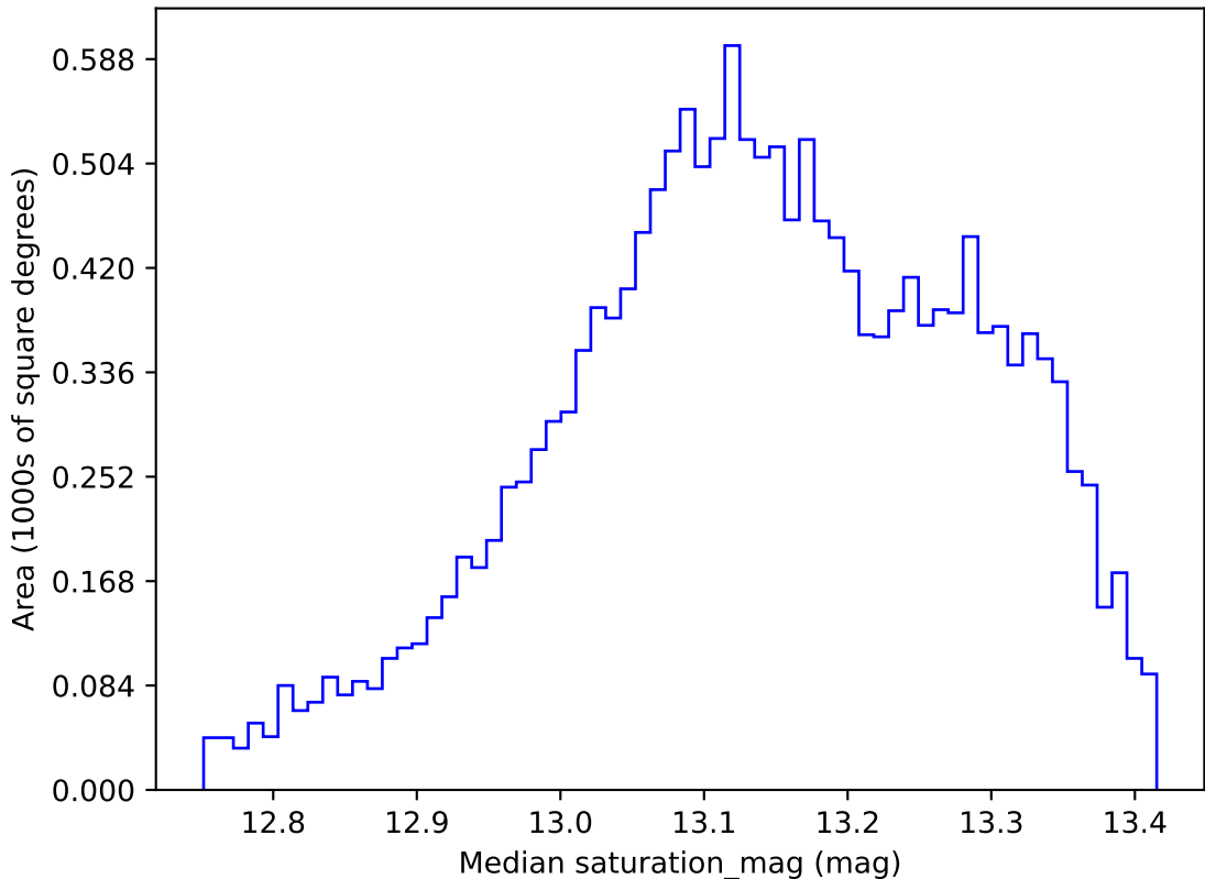
ddf_loaded_half_fl4_v3.4_10yrs WFD y band: Median saturation_mag
