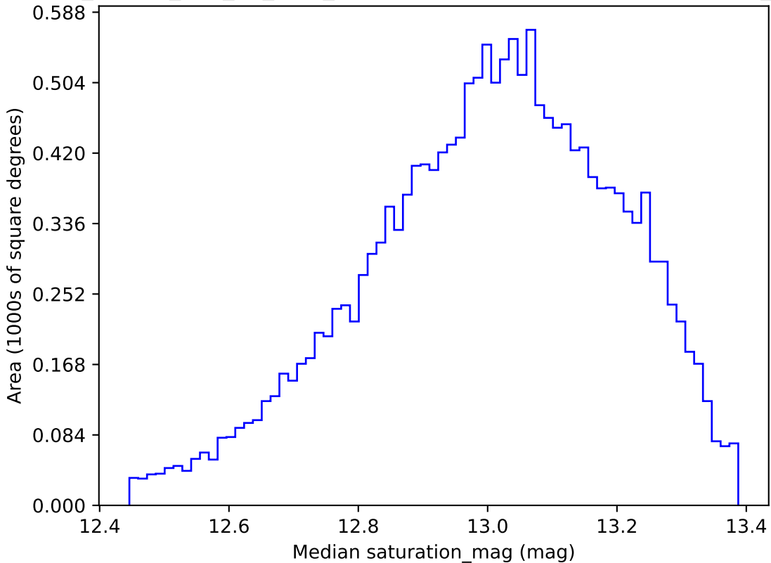
ddf_loaded_half_fl4_v3.4_10yrs WFD u band: Median saturation_mag
