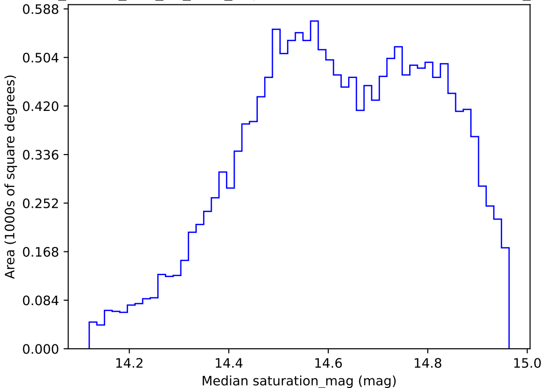
ddf_loaded_half_fl4_v3.4_10yrs WFD r band: Median saturation_mag
