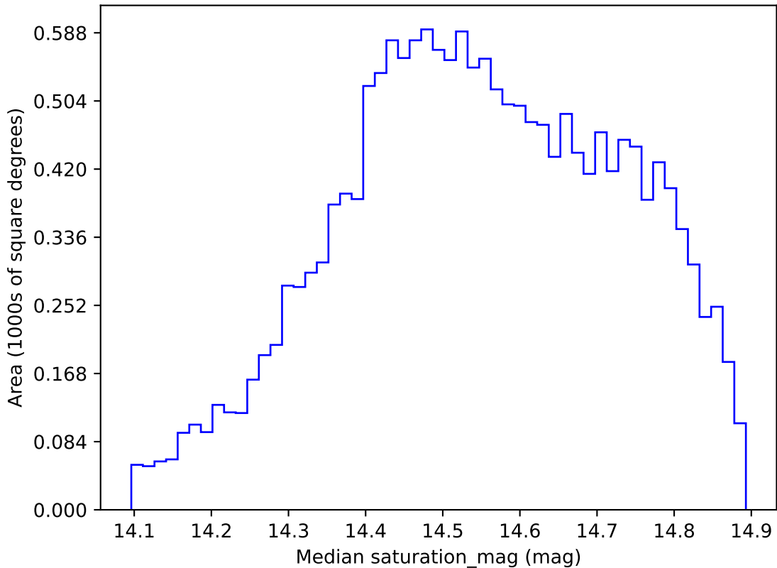
ddf_loaded_half_fl4_v3.4_10yrs WFD i band: Median saturation_mag
