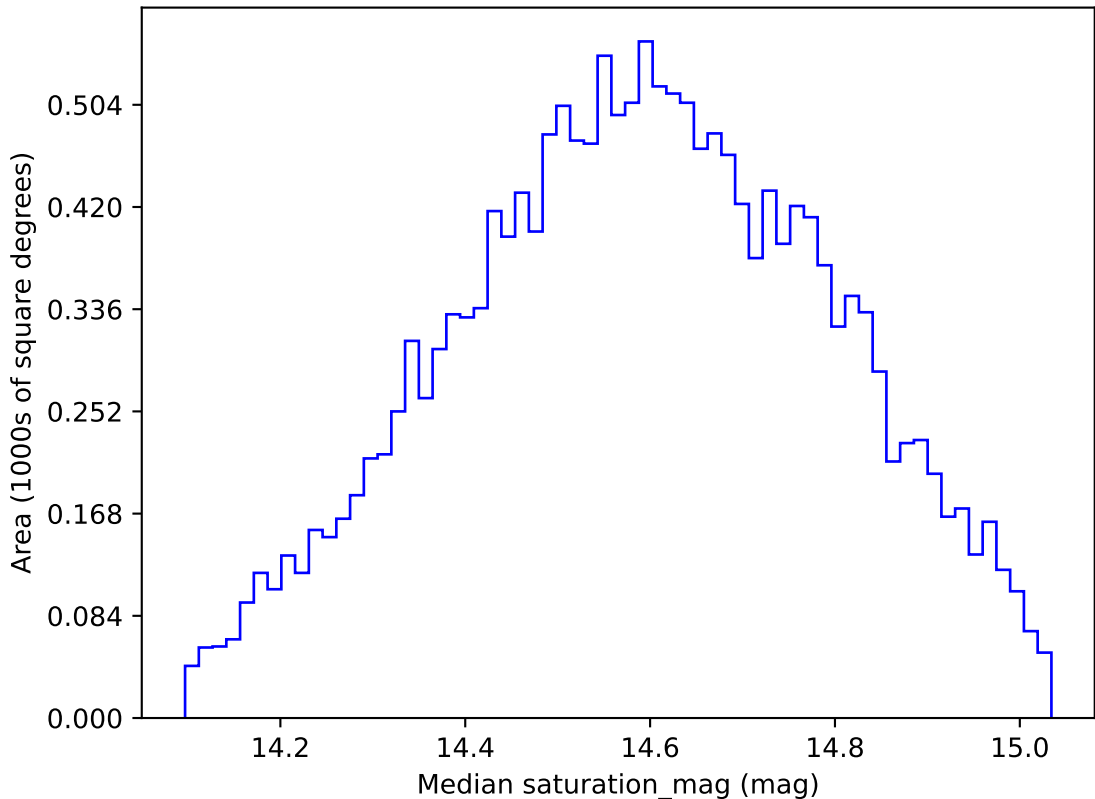
ddf_loaded_half_fl4_v3.4_10yrs WFD g band: Median saturation_mag
