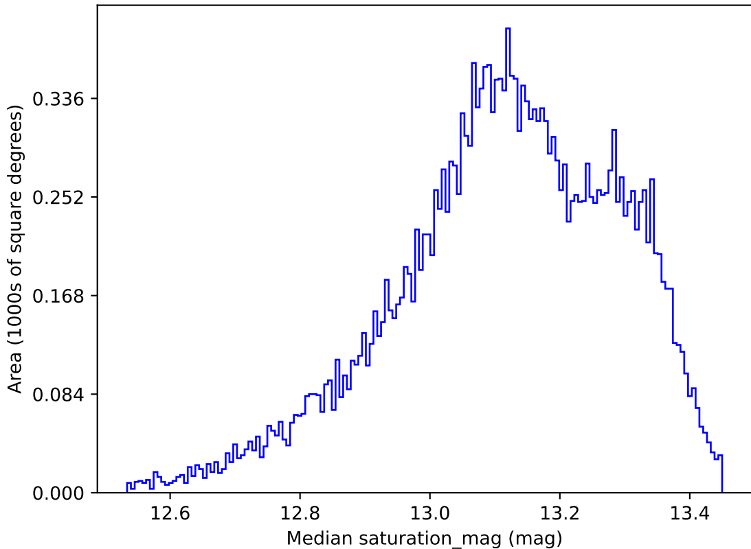
ddf_loaded_half_fl4_v3.4_10yrs All sky y band: Median saturation_mag
