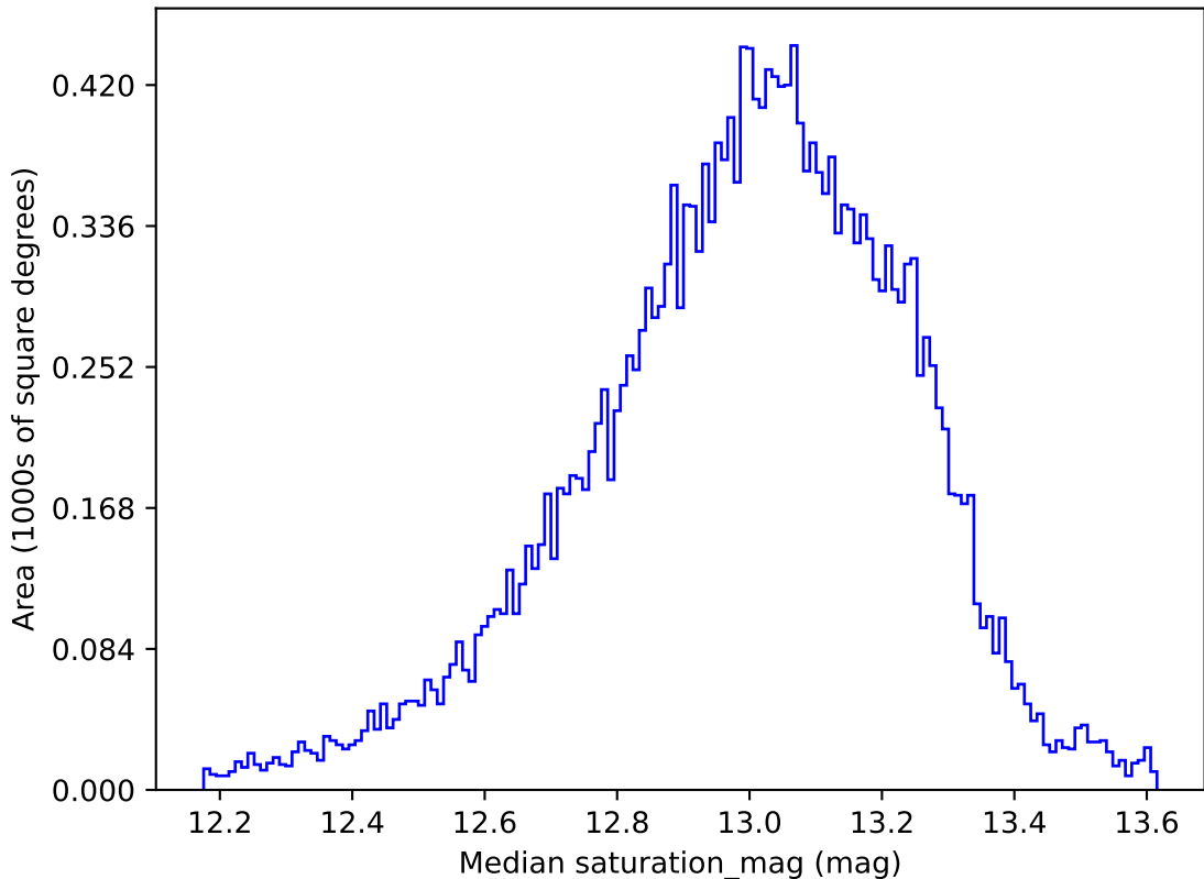
ddf_loaded_half_fl4_v3.4_10yrs All sky u band: Median saturation_mag
