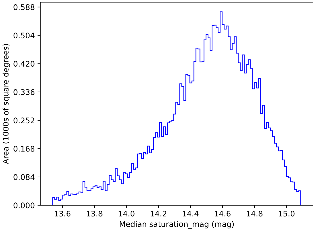
ddf_loaded_half_fl4_v3.4_10yrs All sky g band: Median saturation_mag
