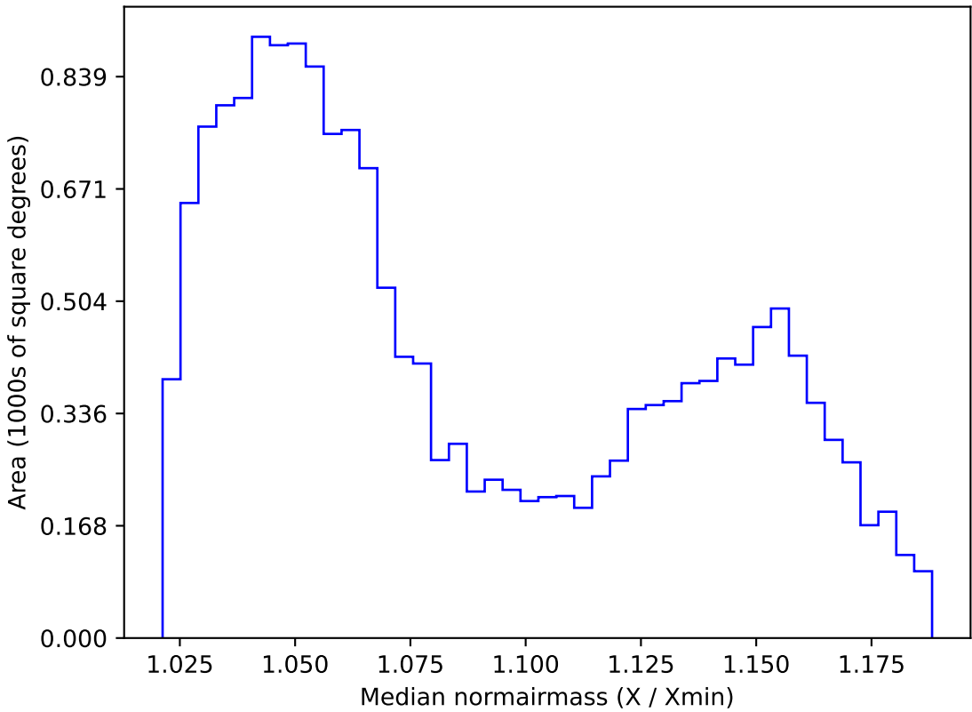
ddf_loaded_half_fl4_v3.4_10yrs WFD z band: Median normairmass
