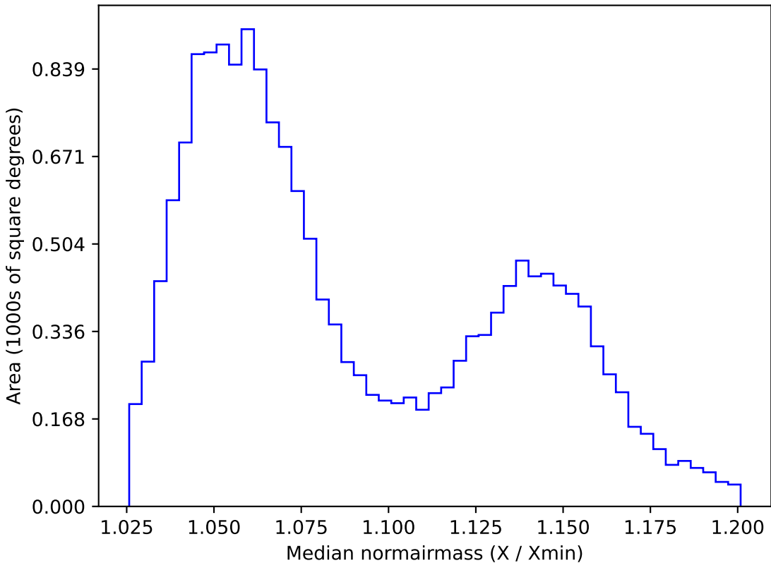
ddf_loaded_half_fl4_v3.4_10yrs WFD y band: Median normairmass
