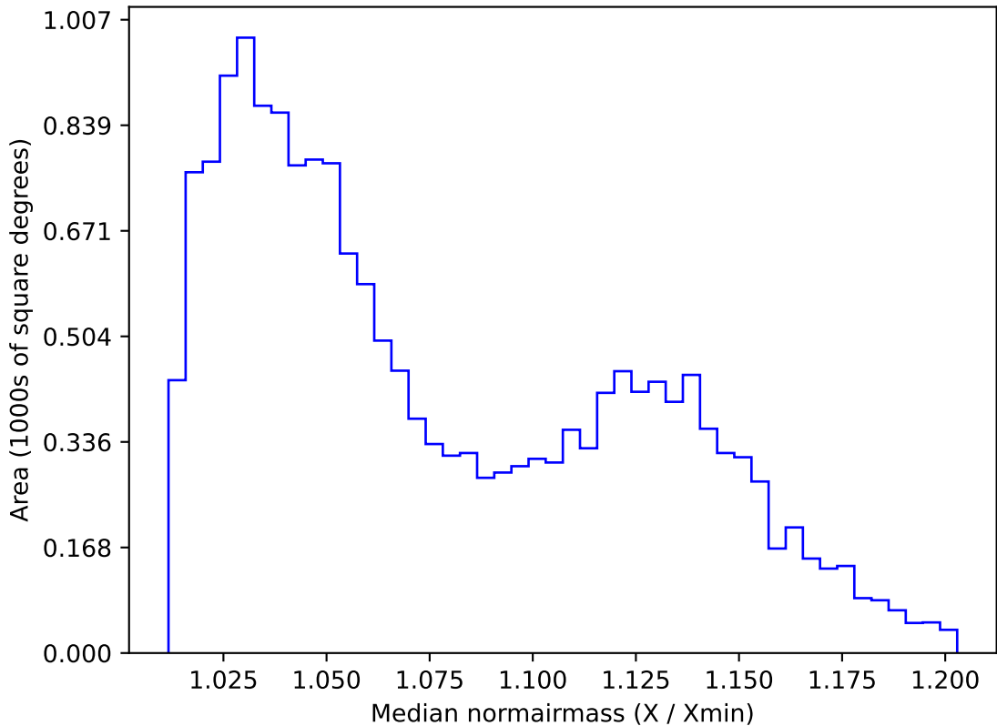
ddf_loaded_half_fl4_v3.4_10yrs WFD u band: Median normairmass
