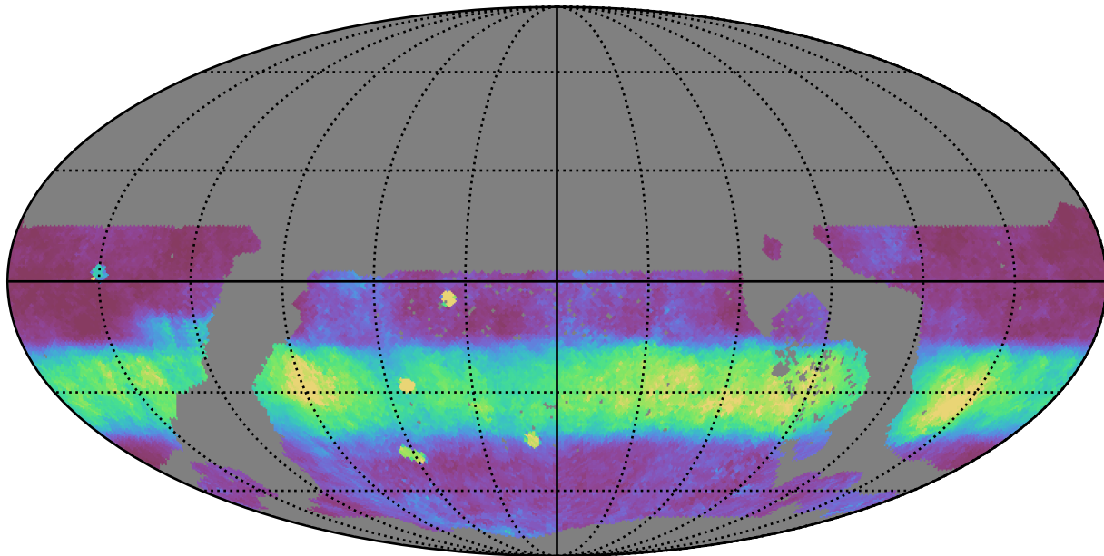
ddf_loaded_half_fl4_v3.4_10yrs WFD r band: Median normairmass
