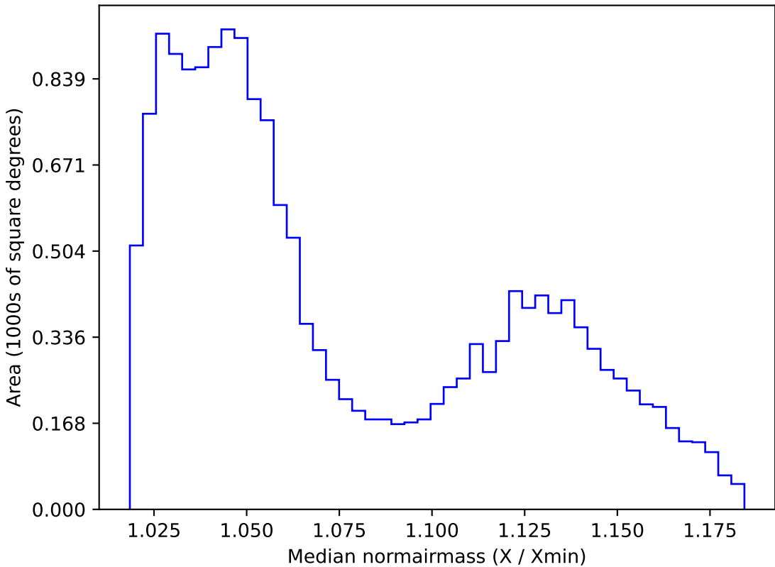
ddf_loaded_half_fl4_v3.4_10yrs WFD r band: Median normairmass
