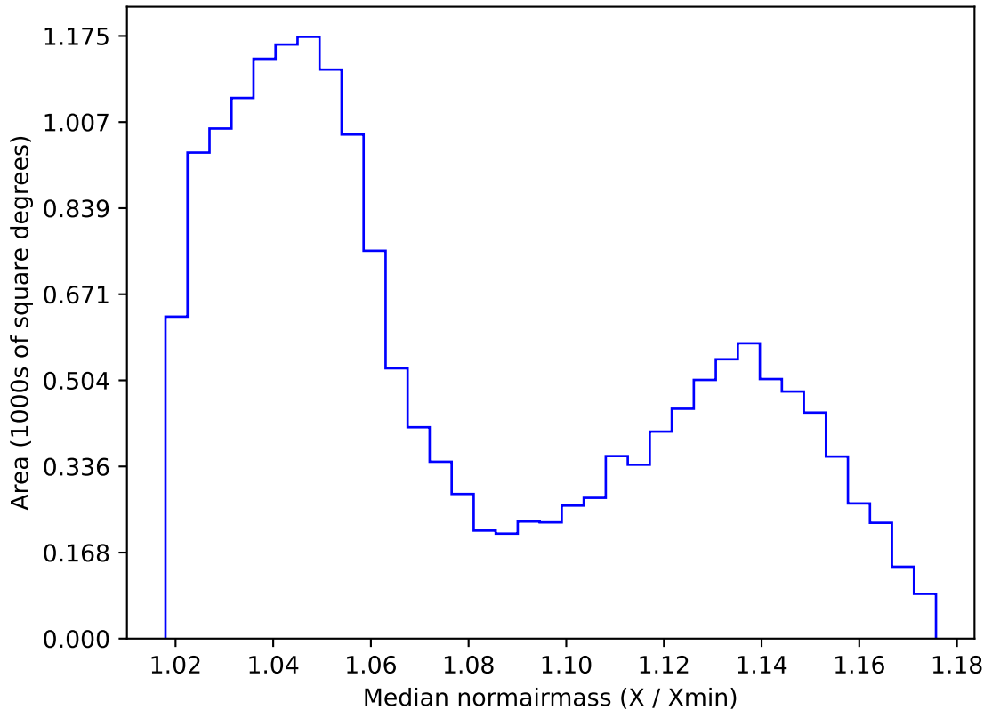
ddf_loaded_half_fl4_v3.4_10yrs WFD i band: Median normairmass
