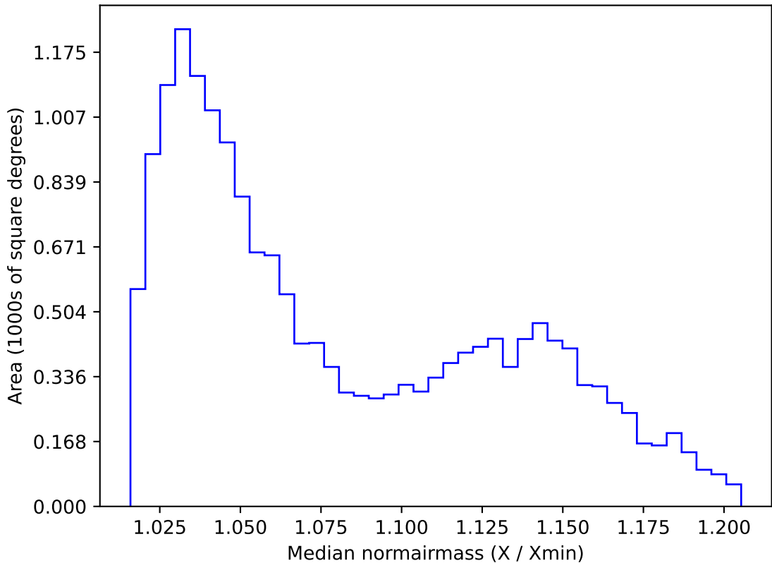
ddf_loaded_half_fl4_v3.4_10yrs WFD g band: Median normairmass
