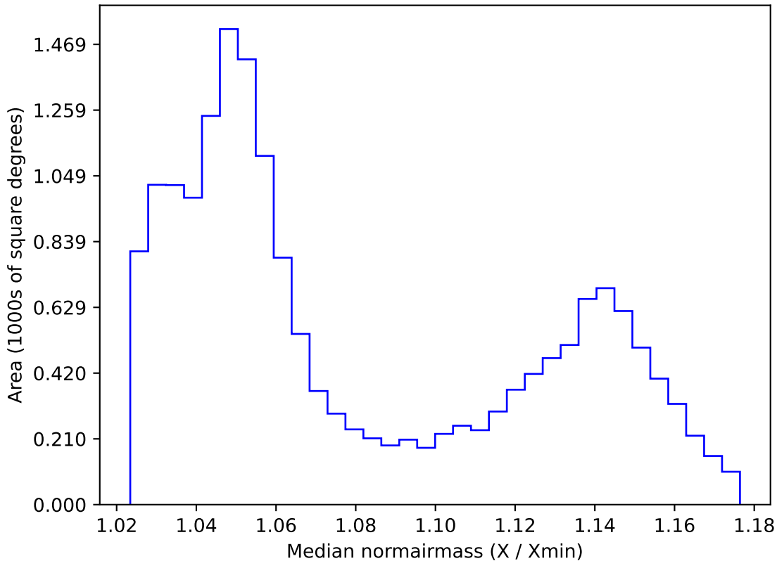
ddf_loaded_half_fl4_v3.4_10yrs WFD all bands: Median normairmass
