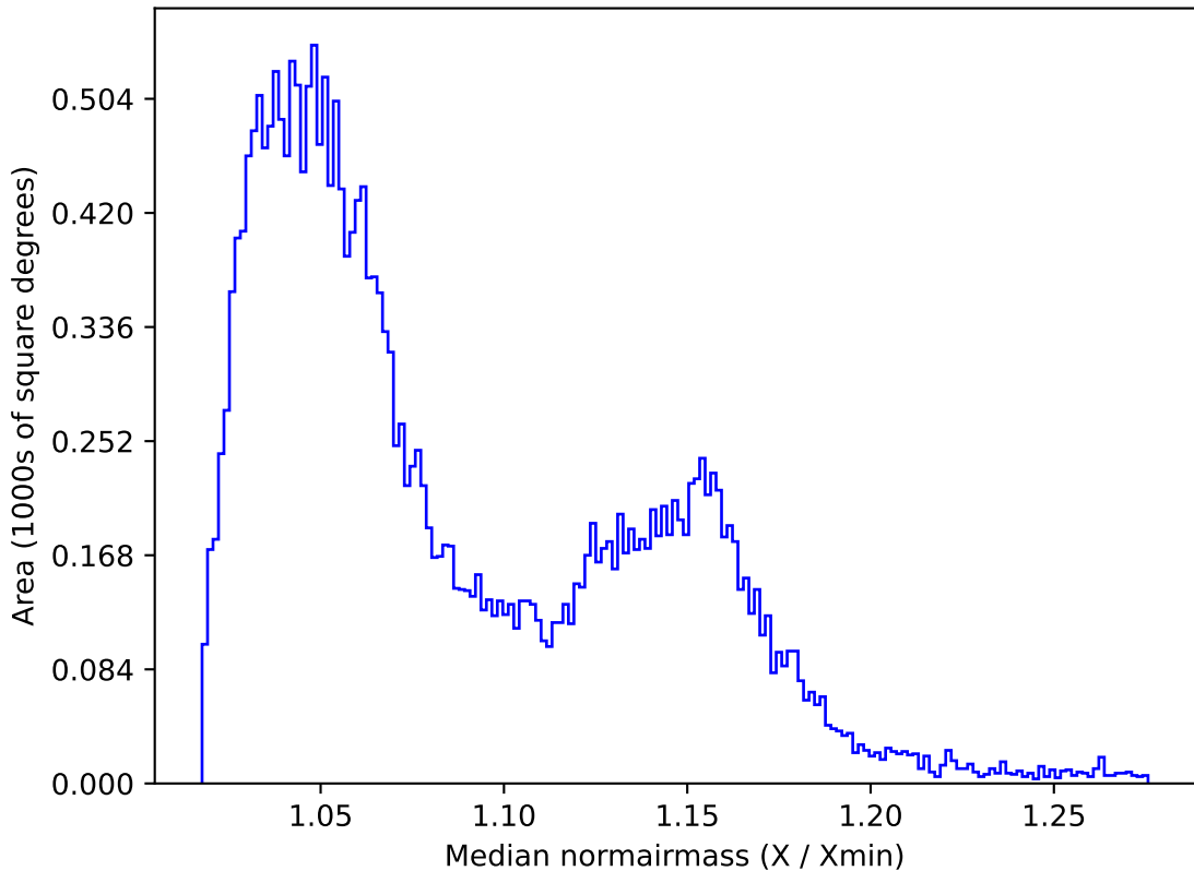
ddf_loaded_half_fl4_v3.4_10yrs All sky z band: Median normairmass
