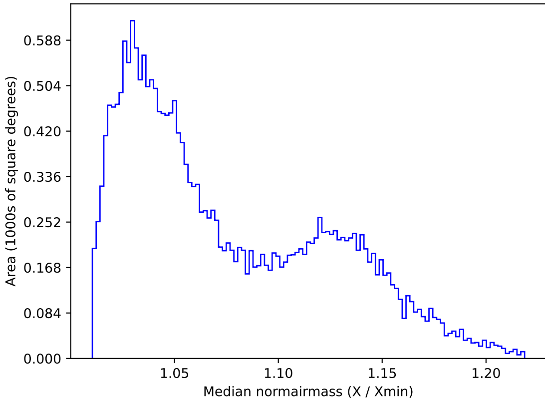
ddf_loaded_half_fl4_v3.4_10yrs All sky u band: Median normairmass
