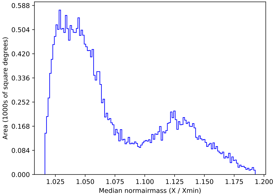
ddf_loaded_half_fl4_v3.4_10yrs All sky r band: Median normairmass
