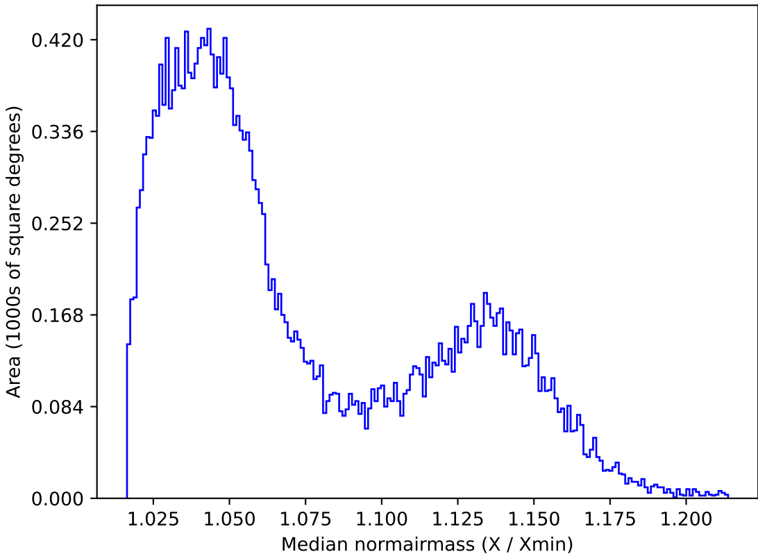
ddf_loaded_half_fl4_v3.4_10yrs All sky i band: Median normairmass
