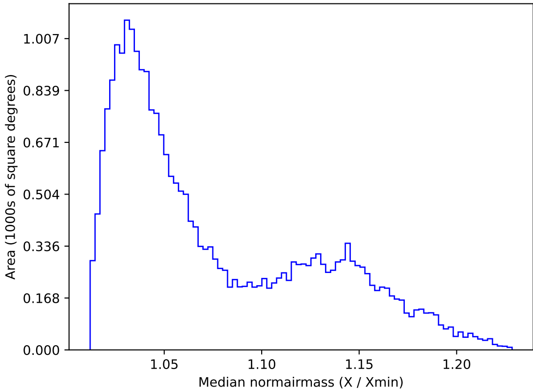
ddf_loaded_half_fl4_v3.4_10yrs All sky g band: Median normairmass
