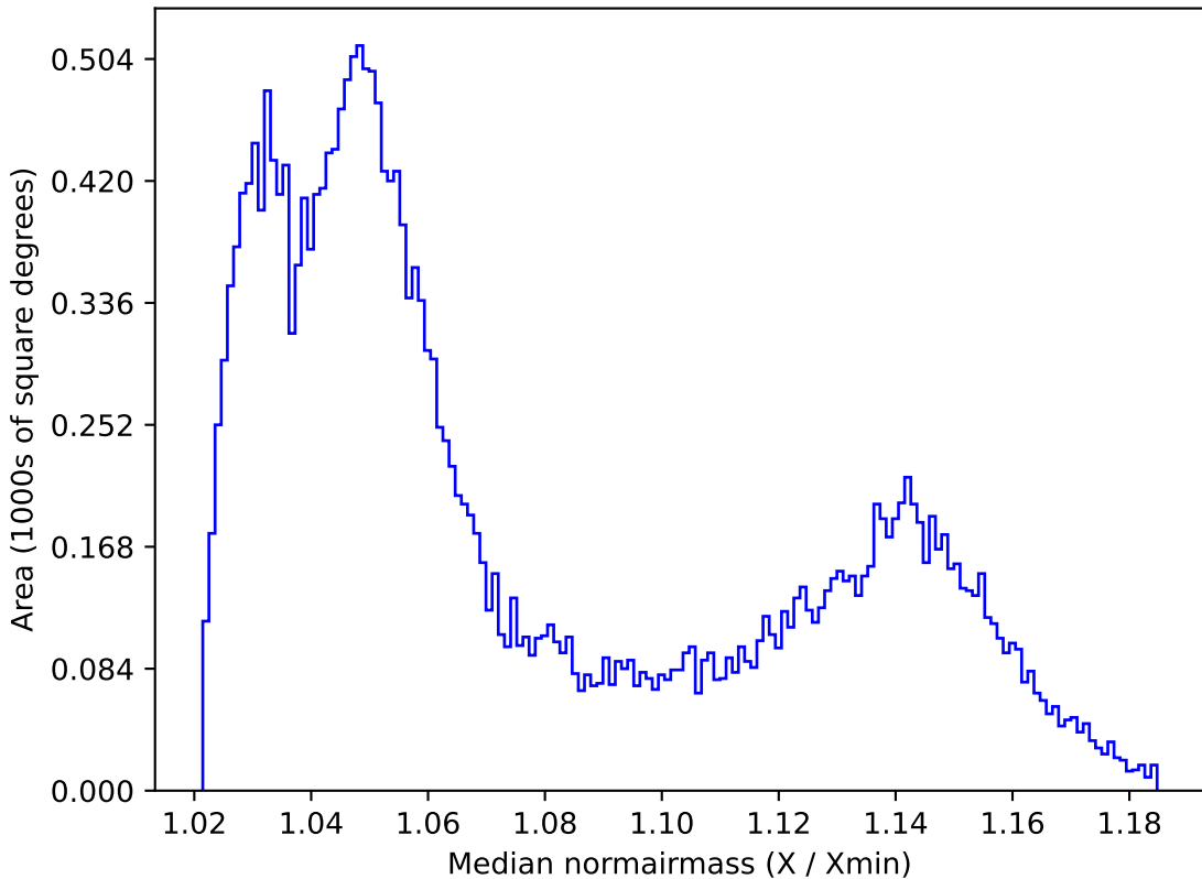
ddf_loaded_half_fl4_v3.4_10yrs All sky all bands: Median normairmass
