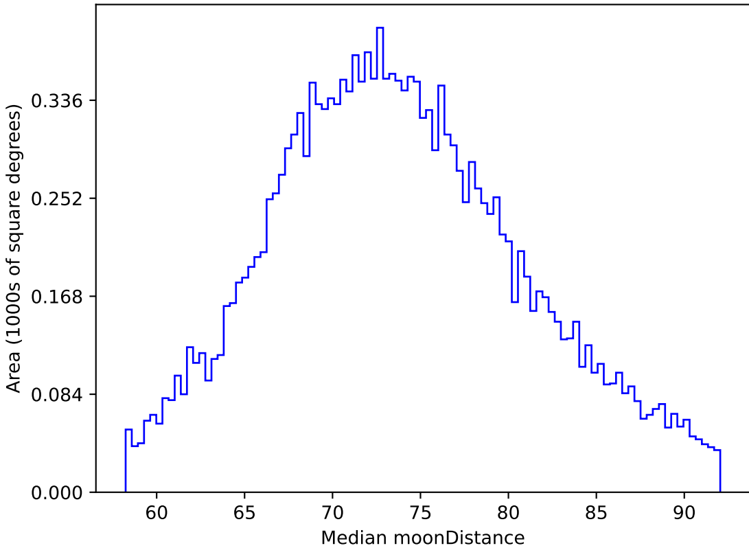
ddf_loaded_half_fl4_v3.4_10yrs WFD z band: Median moonDistance
