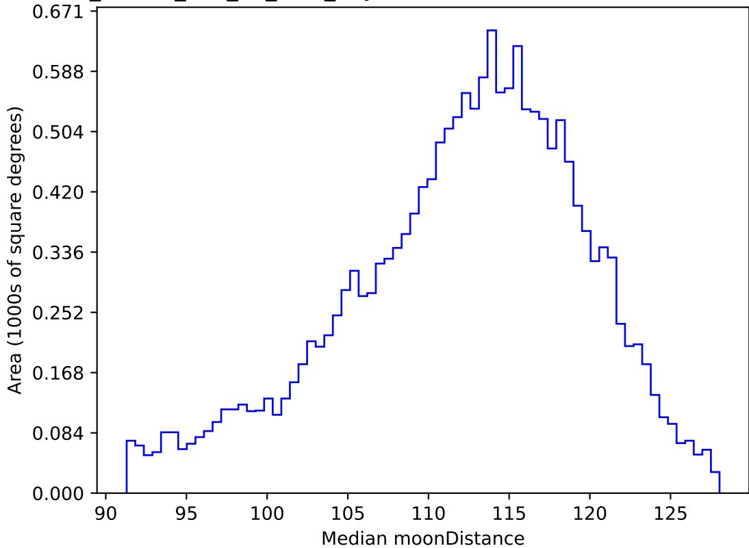
ddf_loaded_half_fl4_v3.4_10yrs WFD r band: Median moonDistance
