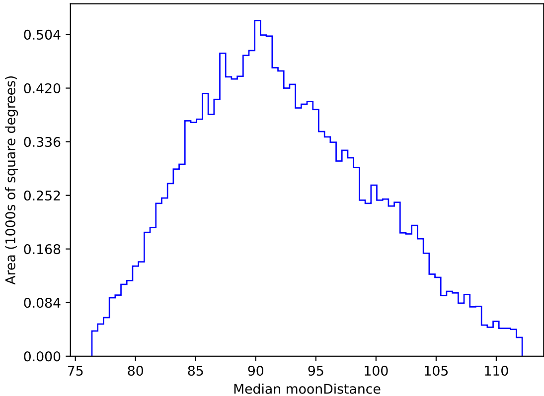
ddf_loaded_half_fl4_v3.4_10yrs WFD i band: Median moonDistance
