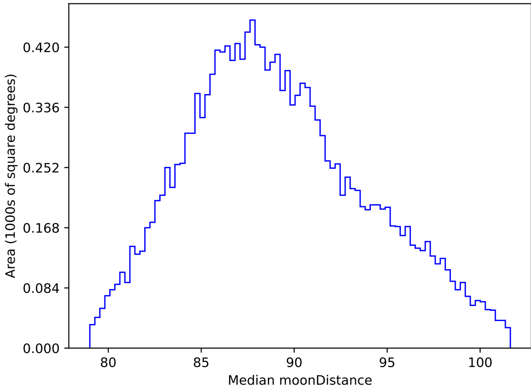
ddf_loaded_half_fl4_v3.4_10yrs WFD all bands: Median moonDistance
