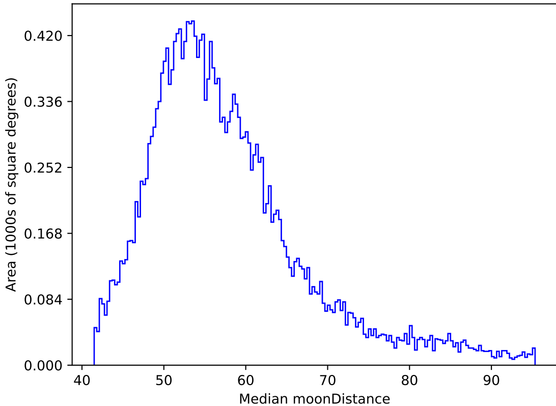
ddf_loaded_half_fl4_v3.4_10yrs All sky y band: Median moonDistance
