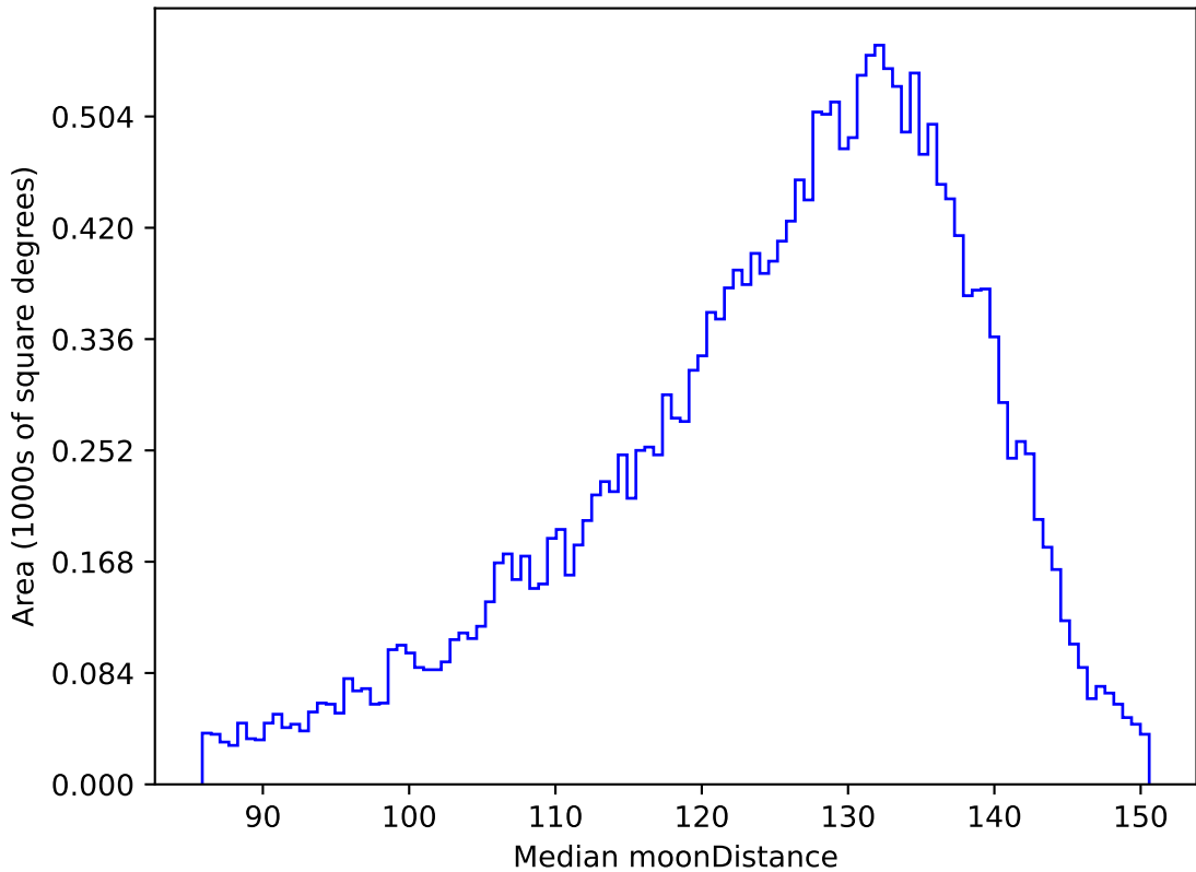
ddf_loaded_half_fl4_v3.4_10yrs All sky u band: Median moonDistance
