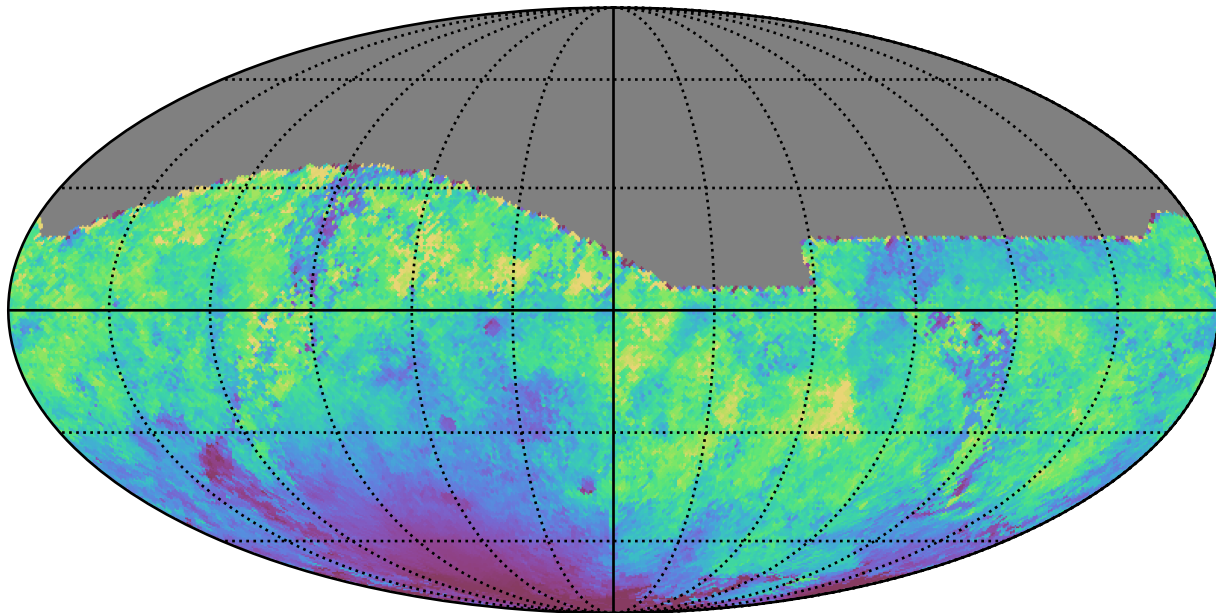
ddf_loaded_half_fl4_v3.4_10yrs All sky r band: Median moonDistance
