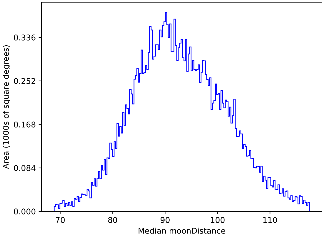
ddf_loaded_half_fl4_v3.4_10yrs All sky i band: Median moonDistance
