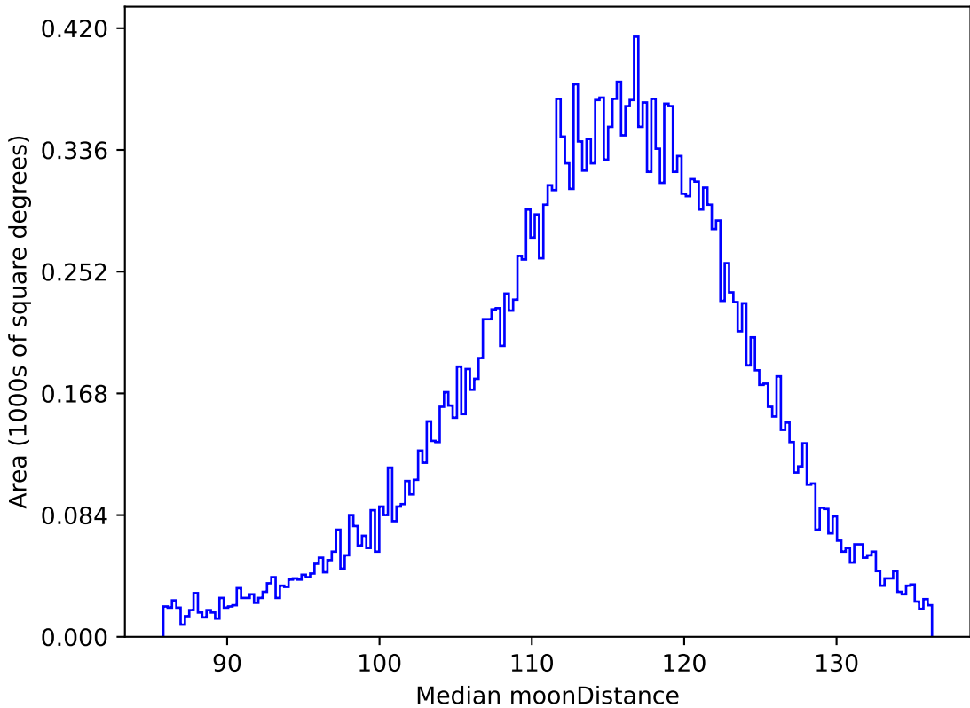
ddf_loaded_half_fl4_v3.4_10yrs All sky g band: Median moonDistance
